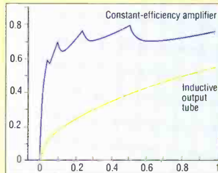
Figure 2. Calculated efficiencies of a conventional IOT and a CEA using an idealized collector model.
