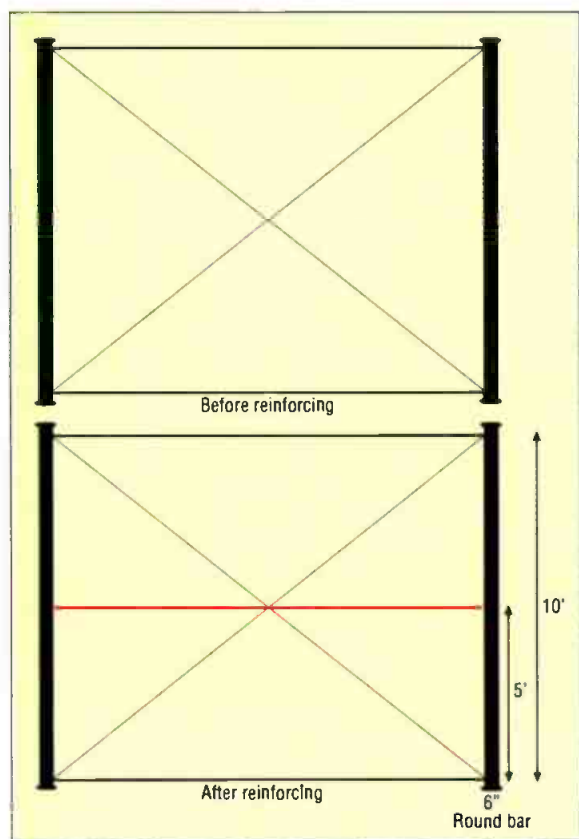
Figure 1. Most tower designs utilize an "X" style bracing system. Additional leg capacity can be obtained by adding reinforcing members. In this example, adding a reinforcing member halfway up the leg section increases the capacity 36%.
