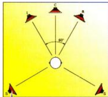
Figure 2. Optimum system speaker placement for HDTV viewing.
