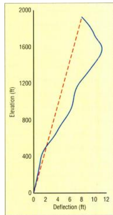
Figure 5. A desirable deflection profile would exhibit even deflection that increases with height (dotted line). This deflection profile is undesirable because of the reduced deflection that occurs starting around 1600 ft.
